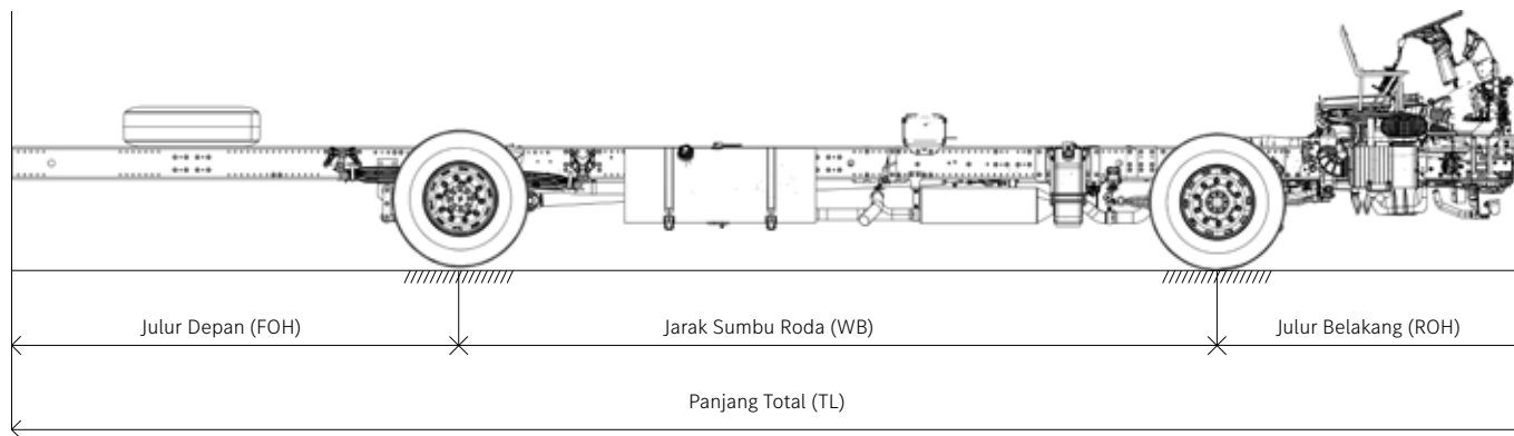
Tampak Samping
