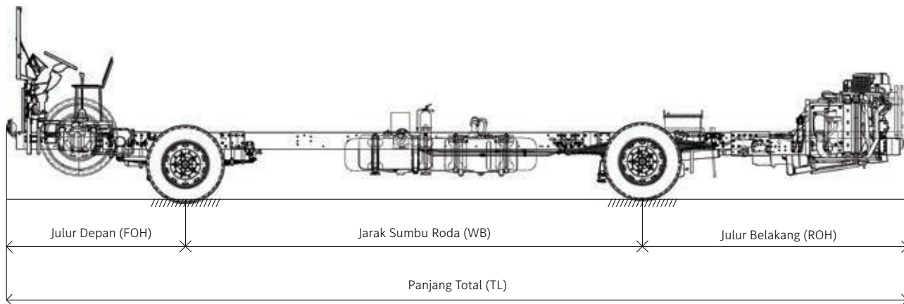
Tampak Samping
